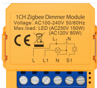
ZIGBEE 3.0
